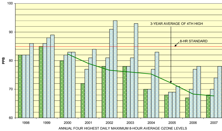
CORPUS CHRISTI FOUR HIGHEST OZONE DAYS TCEQ MONITOR C21 (9860 La Branch)
