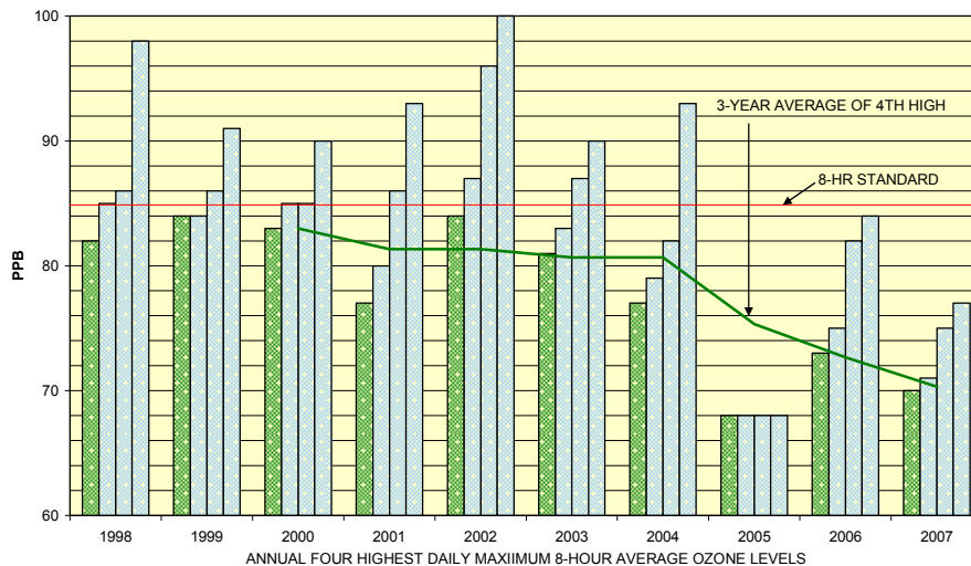
CORPUS CHRISTI FOUR HIGHEST OZONE DAYS TCEQ MONITOR C4 (902 Airport Blvd)
